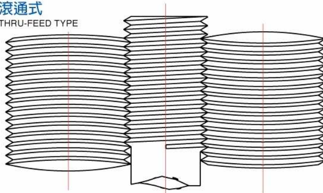
Method of thread rolling
